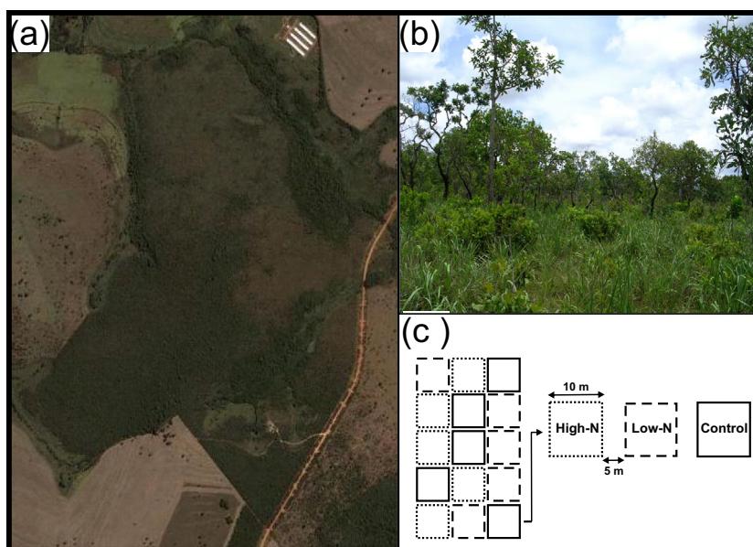
Fig. 1. (a) Aerial view of the study area, (b) view of the cerrado open savanna vegetation and (c) diagram of the experimental plots where nitrogen levels were manipulated.
